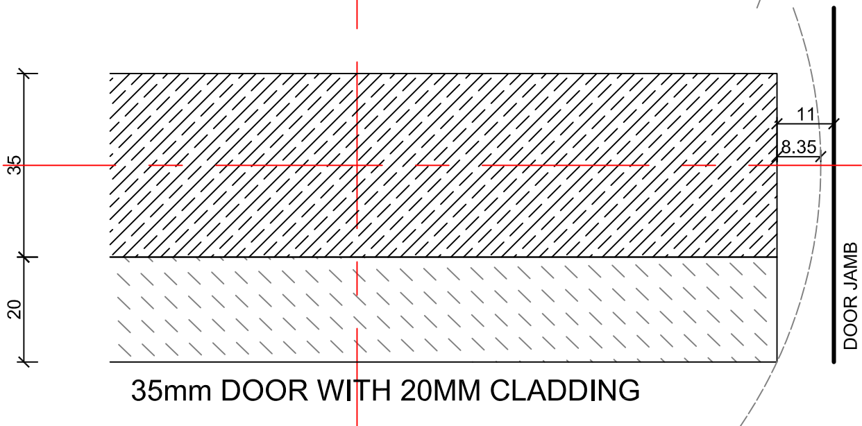
Examples of door clearances required for 80mm backset spring loaded pivot hinge (door jamb is 2.5mm clear of door swing)
